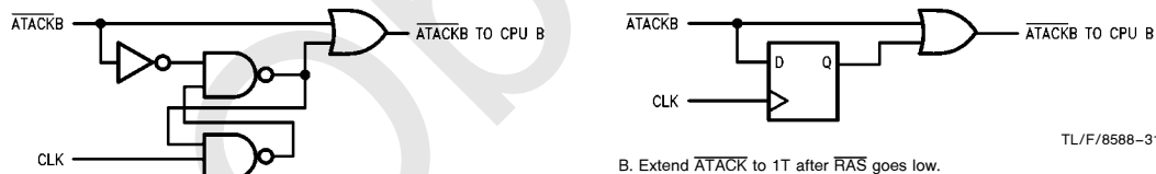
FIGURE 33b. Delayed Port B Access
